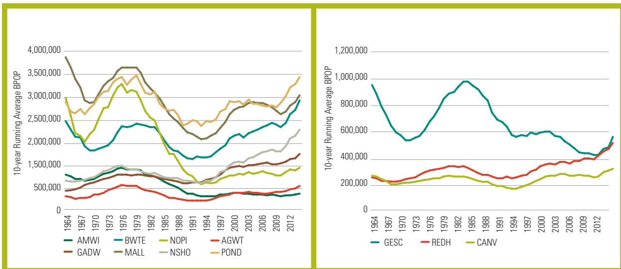
Trends in 10-year running average breeding populations for the seven most common dabbling duck species, 1955-2014 (left panel) and three most common diving duck species (right panel) and ponds from the Waterfowl Breeding Population and Habitat Survey conducted annually across the Prairie Habitat Joint Venture area, 1955-2014.
